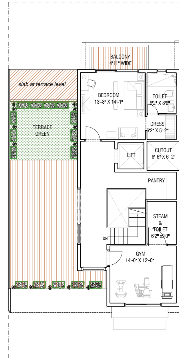
SECOND FLOOR
