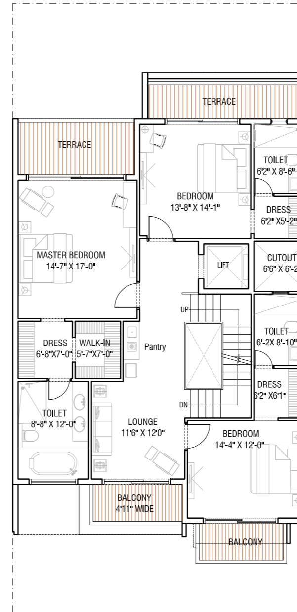
FIRST FLOOR
