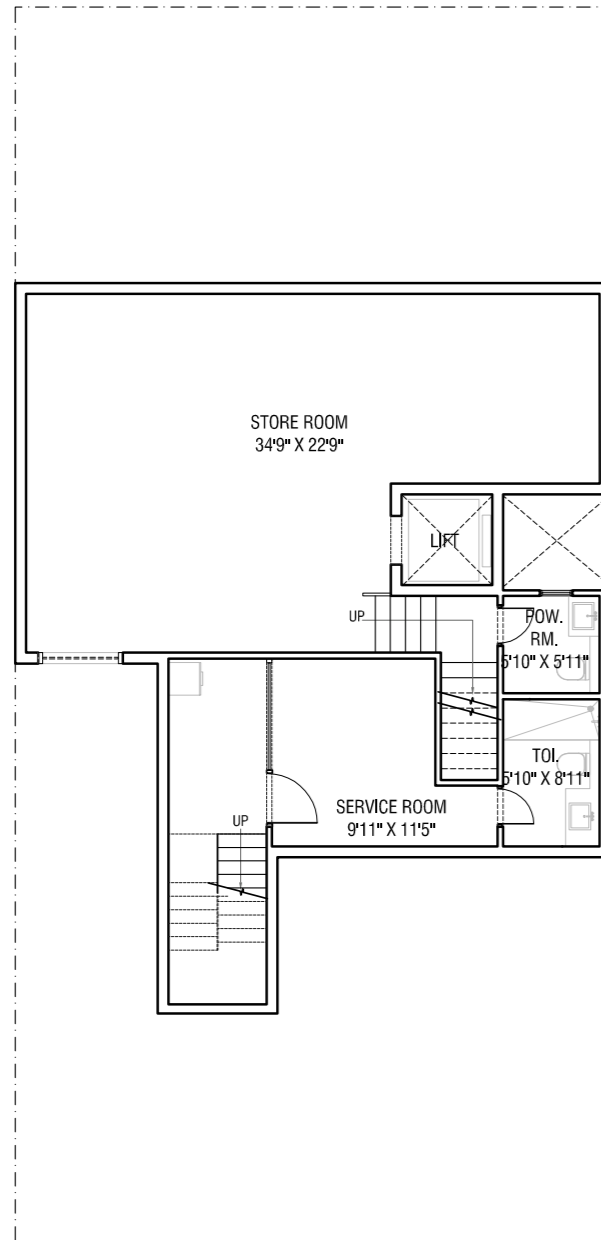
BASEMENT PLAN
