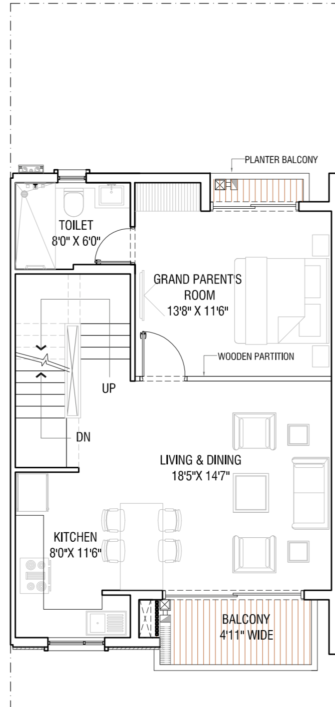
UPPER GROUND FLOOR PLAN
