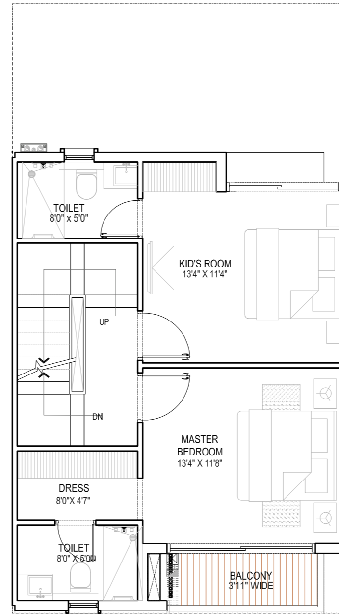
FIRST FLOOR FLAN
