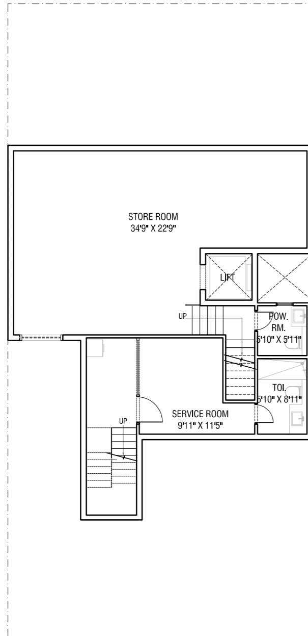
BASEMENT PLAN
