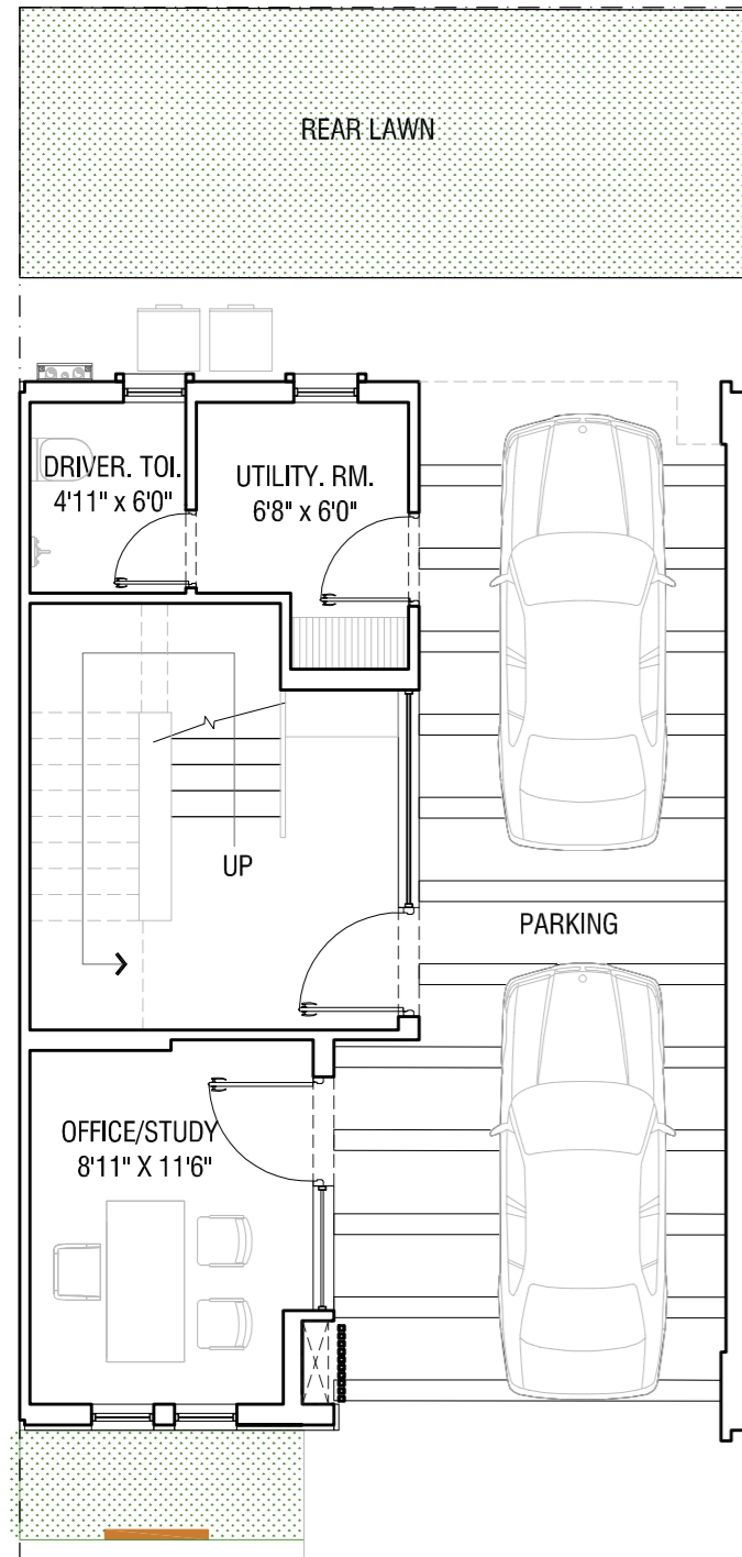
STILT LEVEL PLAN
